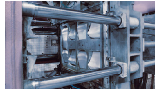
Steam chamber with tool
