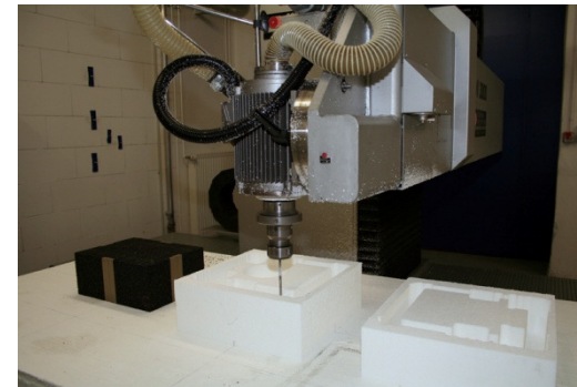
CNC-milling machine
