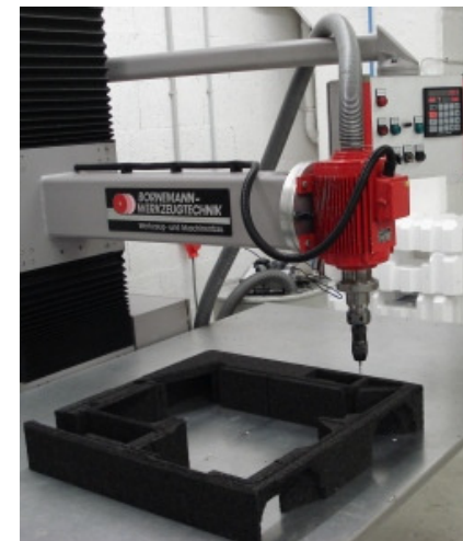
Prototype manufacturing
